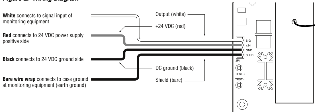
Figure 2. Wiring Diagram
